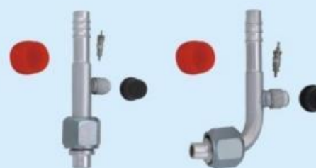
YM-1119 优质接头带R12阀 High-quality adapter with R12 valve 3/8 O 180° with R12 valve
